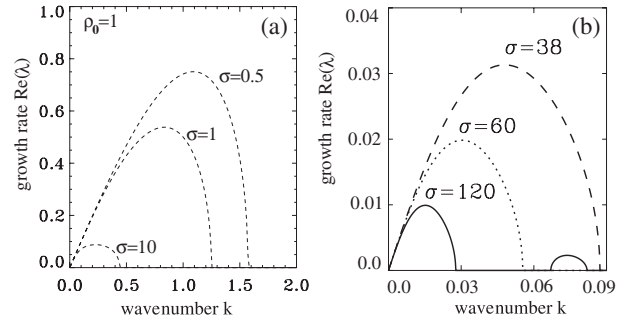
Figure 2. MI gain profile in self-focusing nonlocal media with a Gaussian response function for \rho_0 = 1 (a) and with a generalized Lorentzian response function for n = 2 and \rho_0 = 1.25 (b).
