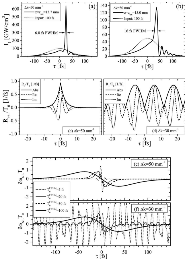
Fig. 2. Numerical simulations of soliton compression of a 100 fs sech pulse in BBO for \lambda_1=1064 nm and N_{eff}=5.3 . The normalized FW intensity at z_{opt} is shown for (a) \Delta k=50 mm -1 (stationary regime) and (b) \Delta k=30 mm -1 (nonstationary regime). The response functions R_{\pm}/T_0 and \delta\omega_{NL}T_0 induced by cascaded SPM for (a) and (b) are shown in (c), (e) and (d), (f), respectively.
