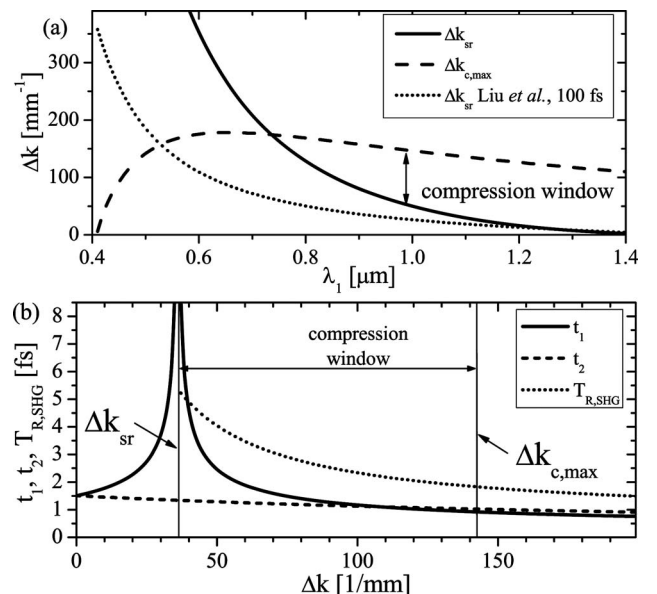
Fig. 1. (a) Compression window Eq. (14) versus \lambda_1 in a BBO. Also \Delta k_{\text{sr}} = 4\pi|d_{12}|/T_0 of [1] for a 100 fs pulse is shown. (b) t_{1,2} and T_{R,\text{SHG}} versus \Delta k for \lambda_1 = 1064 nm.
